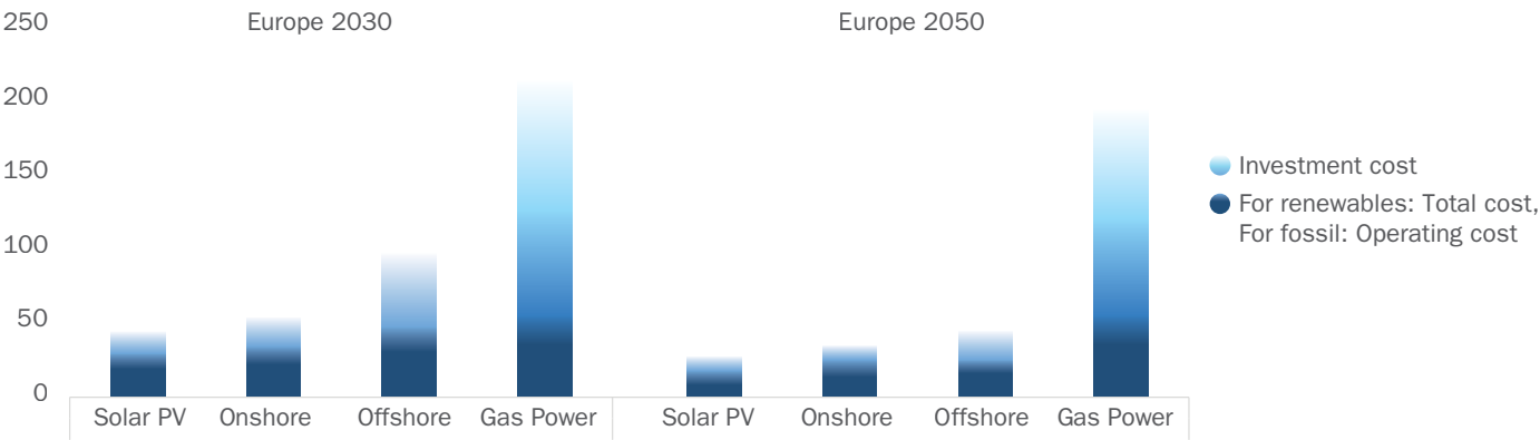
5 Levelised Cost of Energy (LCOE) for different power producing technologies in Europe in 2030 and 2050 (EUR/MWh)
