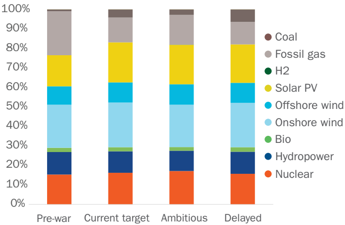
23 Electricity generation share by technology in 2030 for the four scenarios
