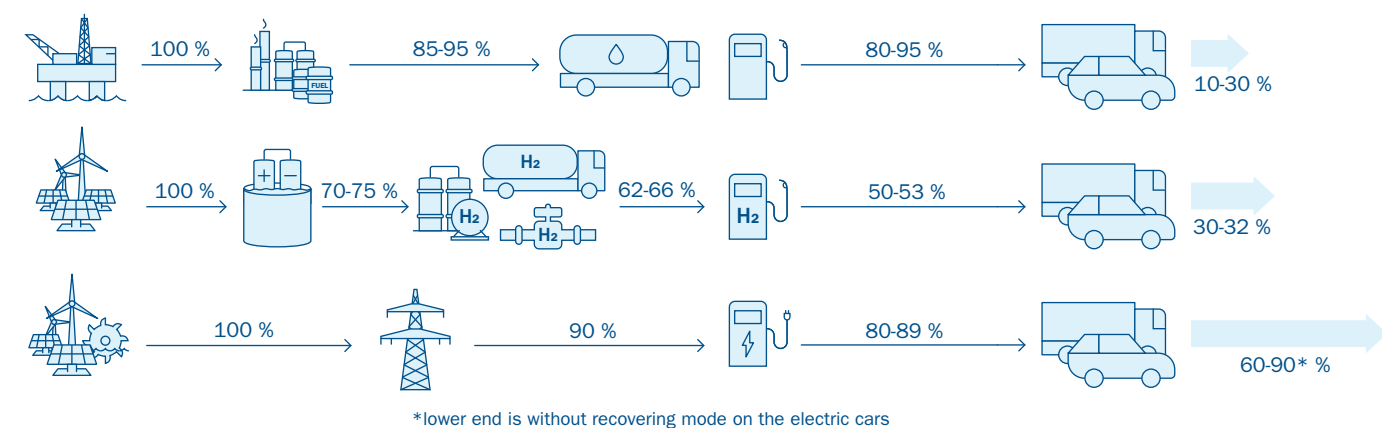
15 Illustration of energy losses for battery electric vehicle (EV), hydrogen fuel cell vehicle (HFCV) and internal combustion engine (ICE)
