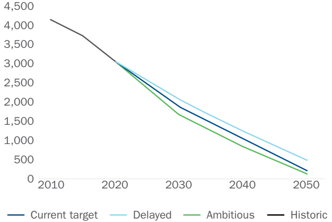
19 Historic CO2 emissions from combustion of fossil fuels for EU27, Norway, Switzerland, and the Balkans (2010 – 2020) along with emission pathways showing different levels of climate ambitions (MtCO2)
