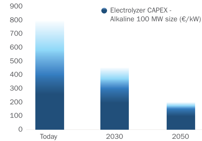
34 Electrolyzer Capex from today to 2050
