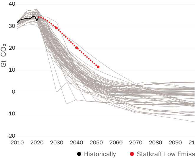
The Low Emissions Scenario compared with emission pathways that correspond to global warming of 1.5 °C
